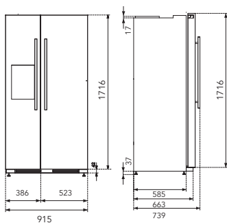
ADAGIO 90 SIDE BY SIDE
