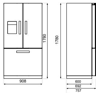
ADAGIO 90 FRENCH-DOOR
