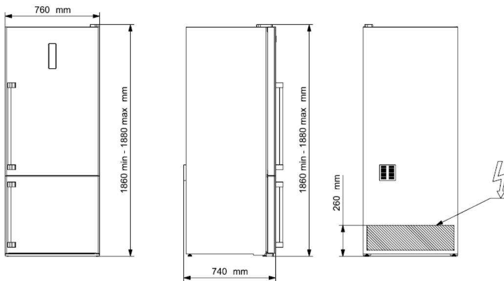
ADAGIO 76 Combi Koelkast
